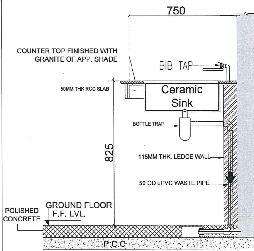
SECTION THROUGH SINK
